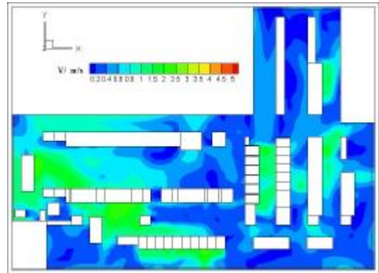
Figure 9. Predicted air velocity distribution after the proposed improvements
