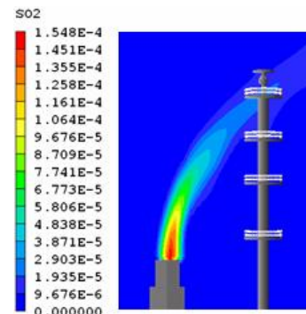
SO 2 Mass Fraction Profiles Impacting the Communication Tower Figure 2: Thermal and Toxic Impact of Turbine Exhaust on Communication Tower
