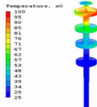
Communication Tower Surface Temperature
